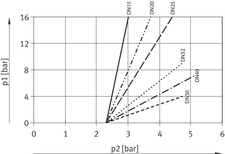
Fig. 4: Operating pressure and medium pressure VZXF-...-A-...-V4V4-...-50
