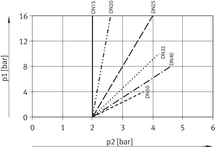
Fig. 3: Operating pressure and medium pressure VZXF-...-A-...-H3B1-...-50
